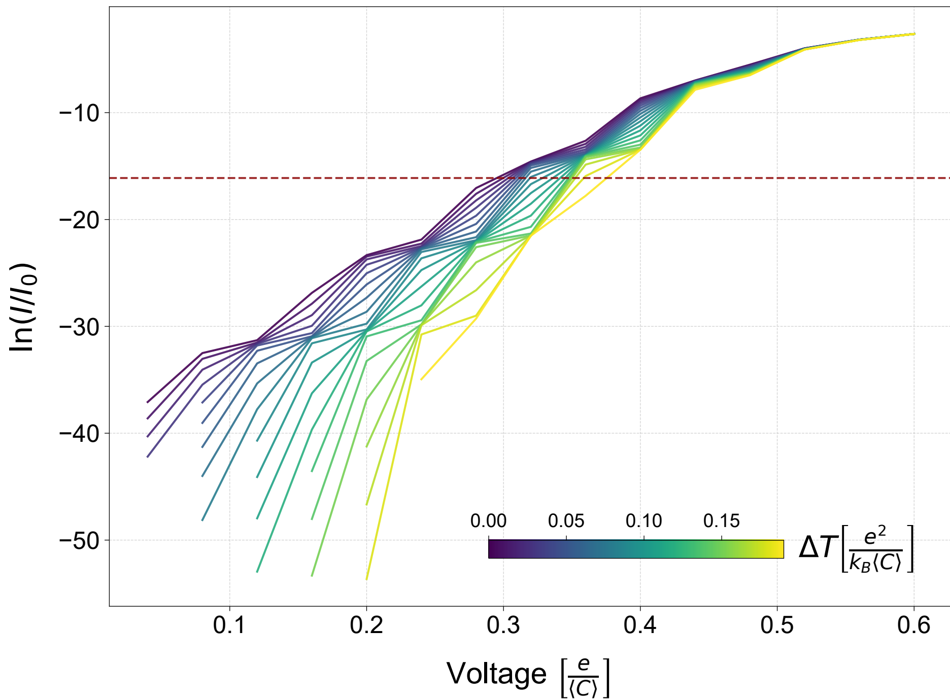
Semi-Log I-V for Fixed Island Temperature T = 0.2E_c
